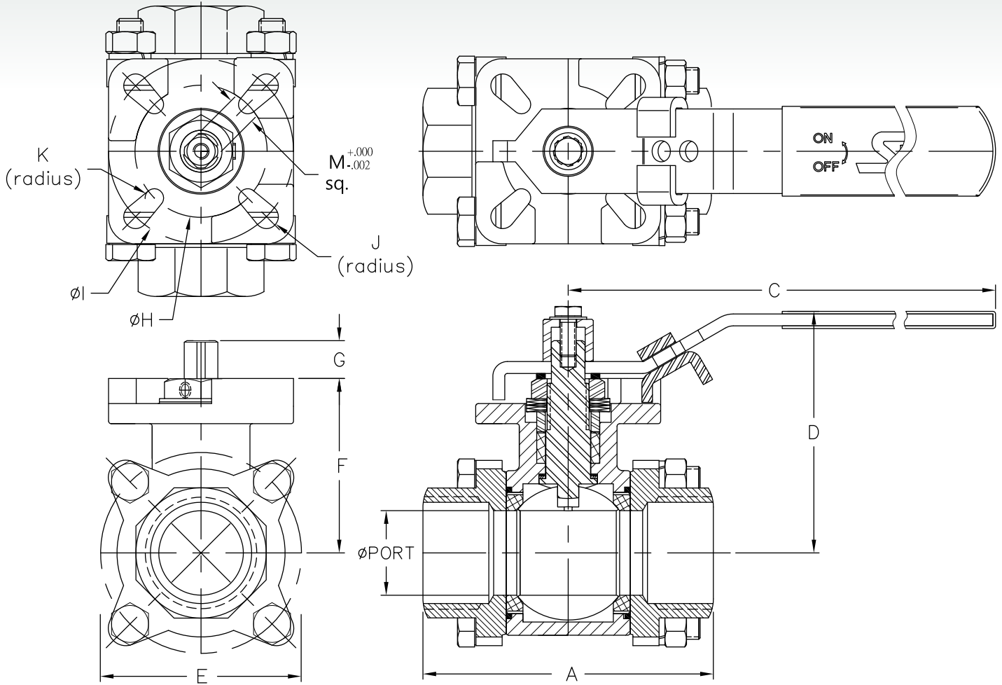
Dimensions (Inches)
